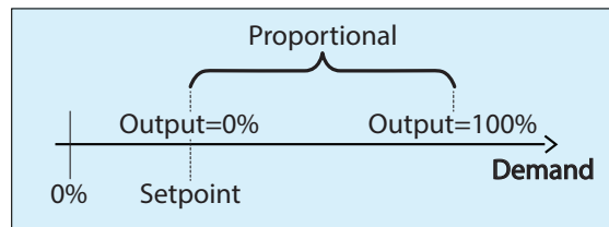
Figure 47 - Reheat Proportional Mode
