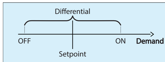
Figure 35 - Valve Differential Control
